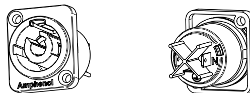
3D VIEW 1 : 1
