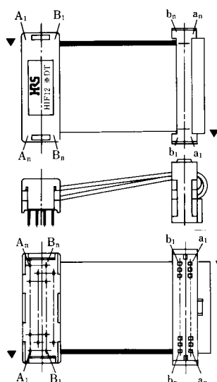
Cable 1 Connection
