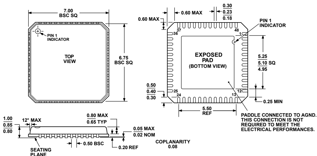
Figure 42. 48-Lead Lead Frame Chip Scale Package [LFCSP_VQ] 7 mm × 7 mm Body, Very Thin Quad (CP-48-1)
