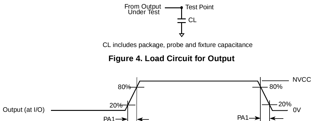
Figure 5. Output Transition Time Waveform
