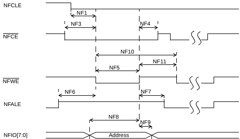
Figure 23. Address Latch Cycle Timing Diagram
