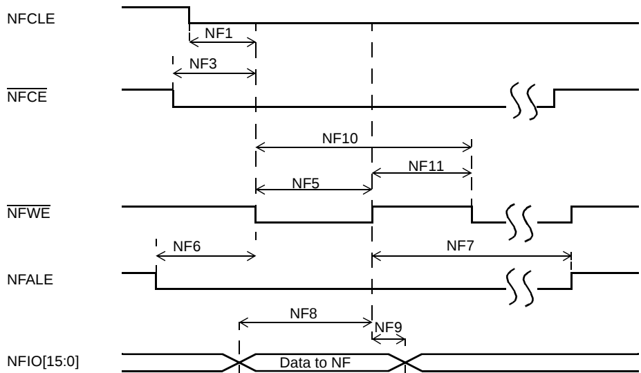
Figure 24. Write Data Latch Cycle Timing Diagram
