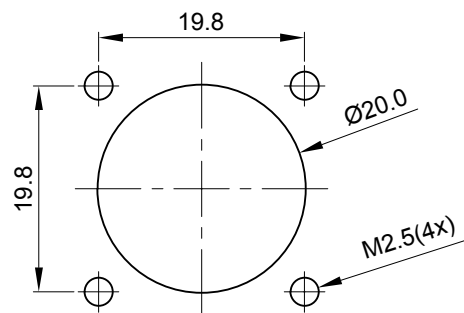
MOUNTING HOLE
