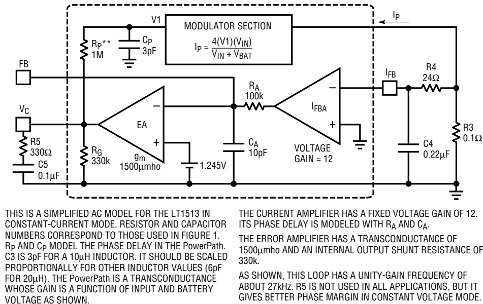
Figure 7. Constant-Current Small-Signal Model
