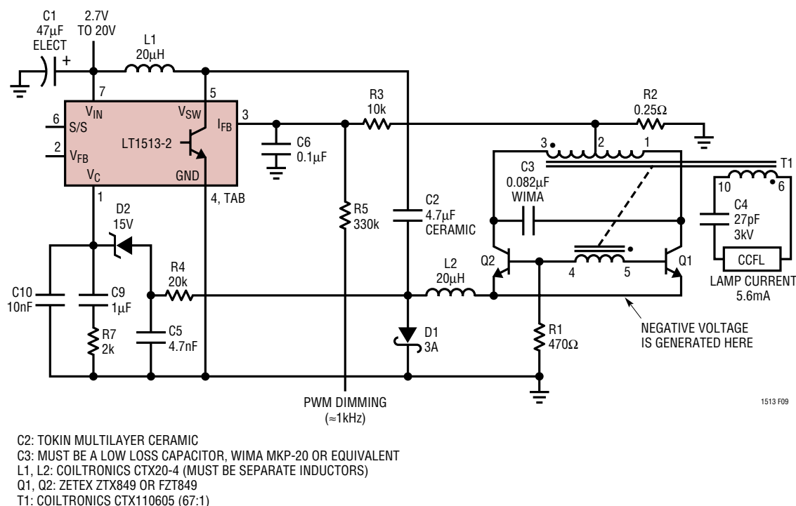
Figure 9. CCFL Power Supply for Floaing Lamp Configuration Operates on 2.7V
