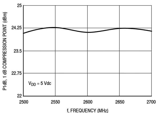
Figure 26. P1dB versus Frequency
