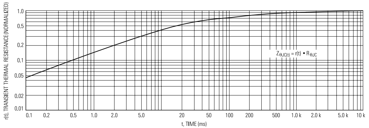
Figure 8. Thermal Response
