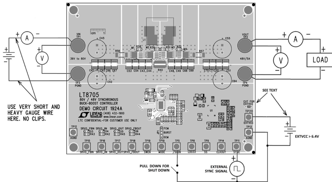
Figure 2. Test Setup
