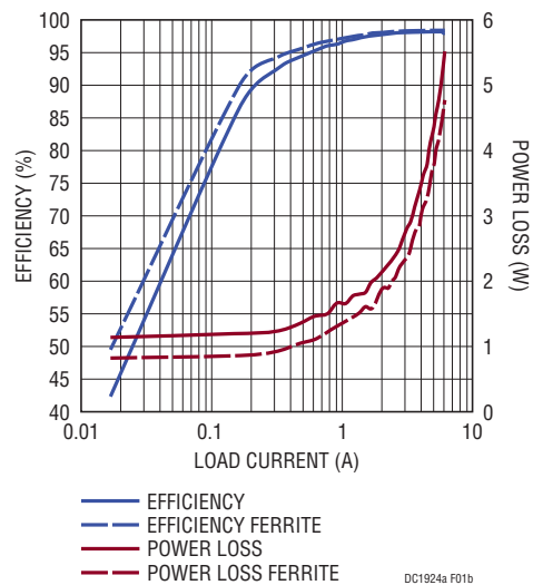
Figure 1b. Efficiency and Power Loss in CCM Buck Mode. V IN = 56V. Dotted Lines Show Increased Efficiency When the Inductor Is Replaced by a Ferrite Core Inductor (Coiltronics SER2918H-223KL)
