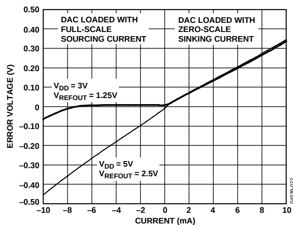
Figure 22. Headroom at Rails vs. Source and Sink
