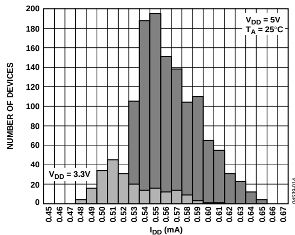
Figure 21. I_{DD} Histogram
