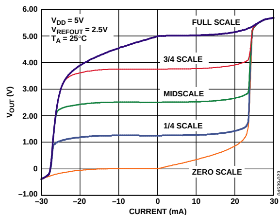
Figure 23. Source and Sink Capability—AD5660-2/AD5660-3
