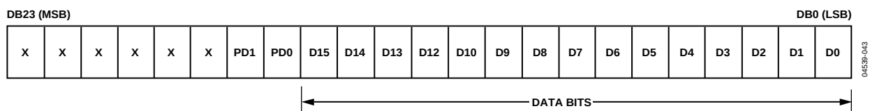
Figure 43. AD5660 Input Register Contents
