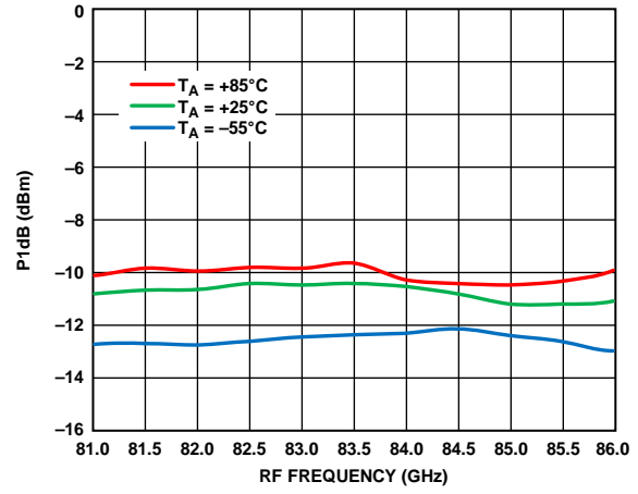
Figure 95. Input P1dB vs. RF Frequency at Various Temperatures, LO = 2 dBm, IF = 2000 MHz, V DLNA = 3 V
