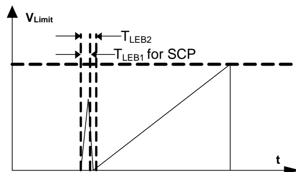
Figure 10: Leading-Edge Blanking
