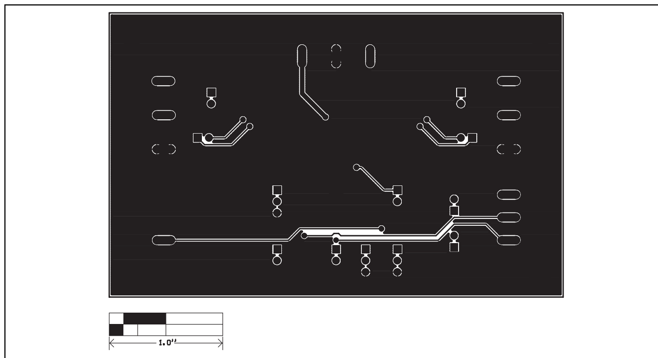
Figure 4. MAX6791 EV Kit PC Board Layout—Solder Side
