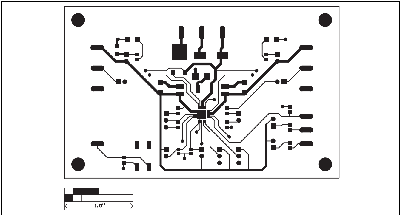
Figure 3. MAX6791 EV Kit PC Board Layout—Component Side
