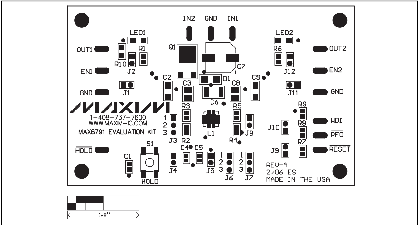
Figure 2. MAX6791 EV Kit Component Placement Guide—Component Side
