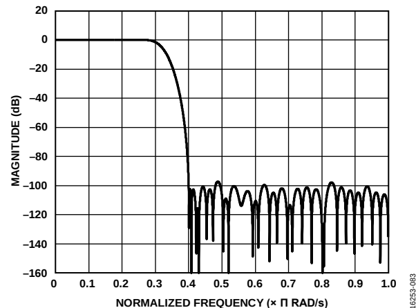
Figure 84. TB1 Filter Response
