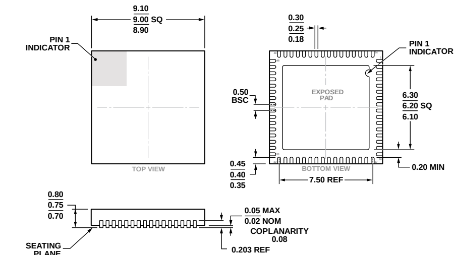
COMPLIANT TO JEDEC STANDARDS MO-220-WMMD Figure 118. 64-Lead Lead Frame Chip Scale Package [LFCSP] 9 mm × 9 mm Body and 0.75 mm Package Height (CP-64-17) Dimensions shown in millimeters
