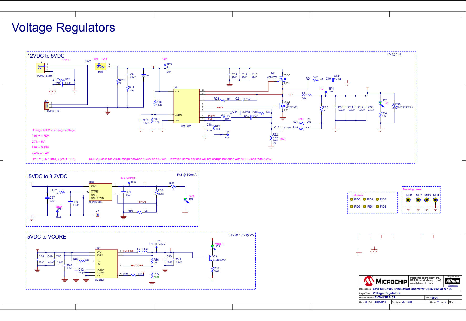
FIGURE A-8: EVB-USB7002 VOLTAGE REGULATORS
