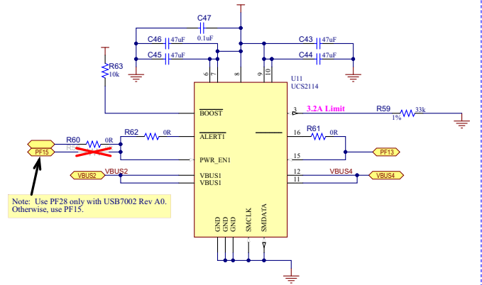
UCS2114 Power Switch For Port2 and Port4
