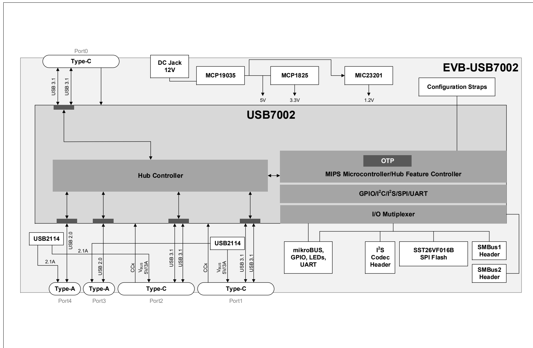
FIGURE 1-1: EVB-USB7002 BLOCK DIAGRAM
