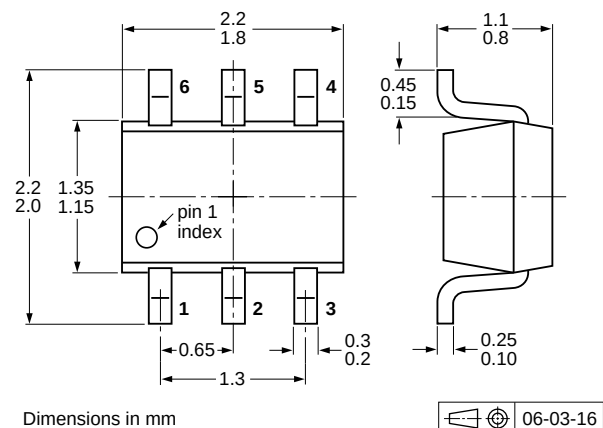
Fig 17. Package outline PUMD9 (SOT363)
