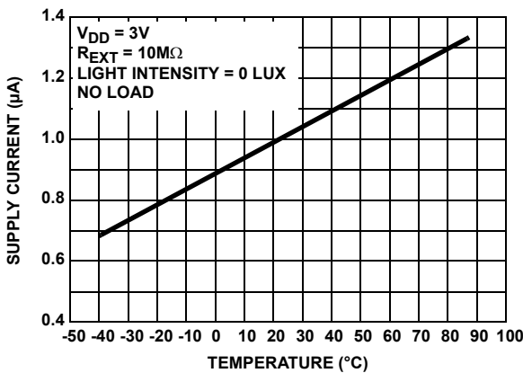
FIGURE 11. SUPPLY CURRENT vs TEMPERATURE AT 0 LUX
