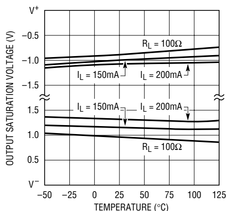
Output Saturation Voltage vs Temperature, V_S = \pm 6\text{V}
