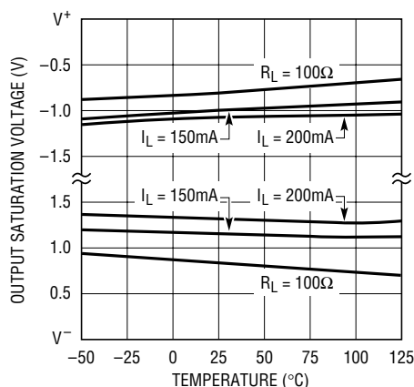
Output Saturation Voltage vs Temperature, V_S = \pm 2.5\text{V}
