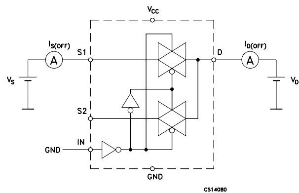
Figure 5. Off leakage
