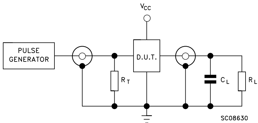
Figure 7. Test circuits
