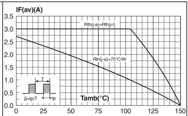
Figure 2. Average forward current versus ambient temperature ( \delta = 0.5 )
