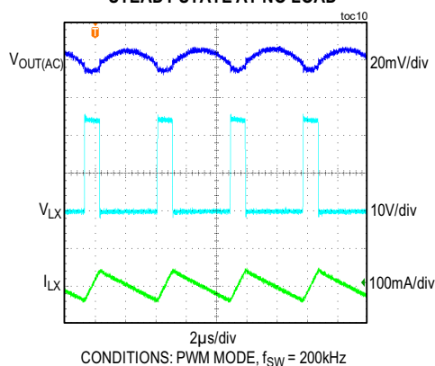
MAX17671F, 5V OUTPUT STEADY STATE AT NO LOAD
