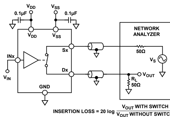
Figure 29. Bandwidth
