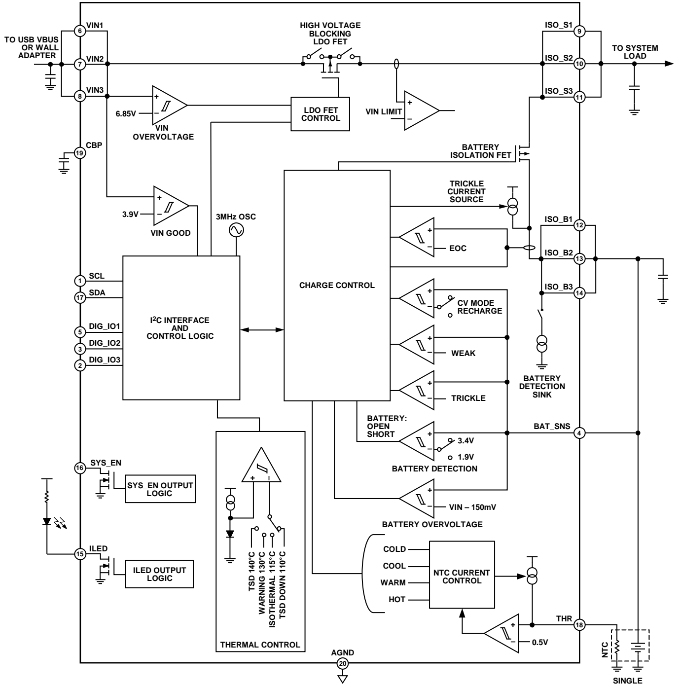
Figure 29. Block Diagram
