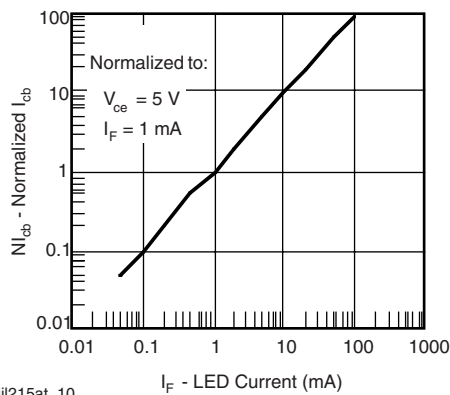
iii215at_10
