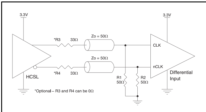
Figure 2E. CLK/nCLK Input Driven by a 3.3V HCSSL Driver
