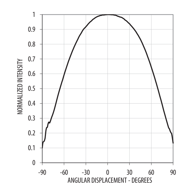
Figure 5: Radiation Pattern
