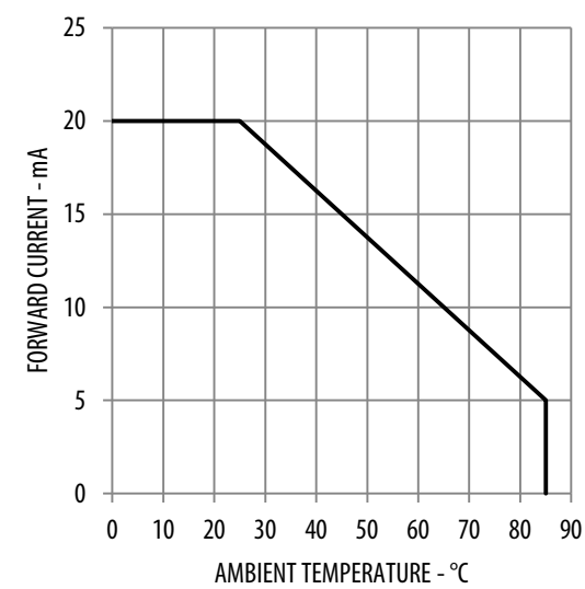
Figure 10: Derating Curve
