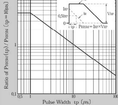
Repetitive Surge Reverse Power Capability
