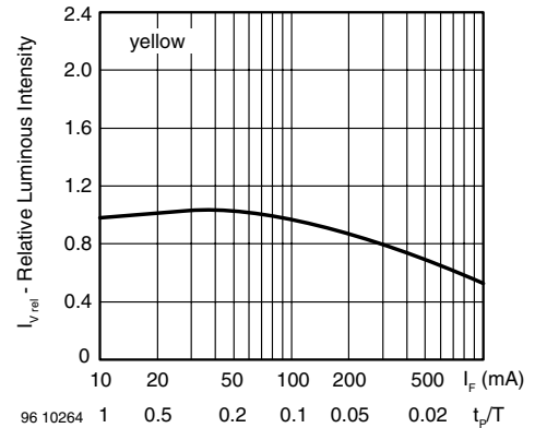
Figure 4. Rel. Lumin. Intensity vs. Forw. Current/Duty Cycle
