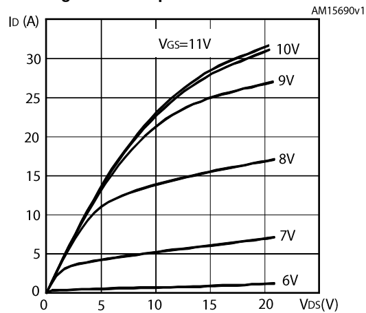
Figure 10: Output characteristics
