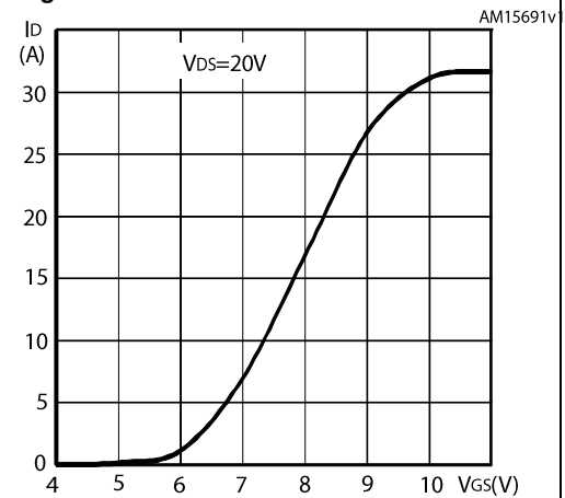
Figure 11: Transfer characteristics
