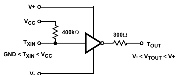
FIGURE 2. TRANSMITTER
