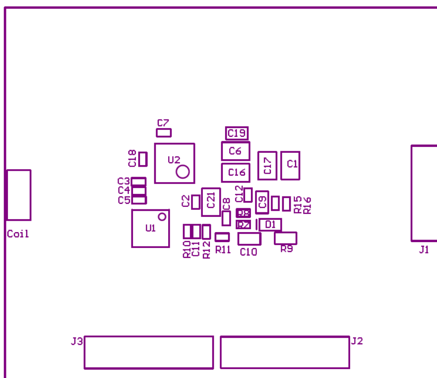
Figure 3: Mechanical13 layer
