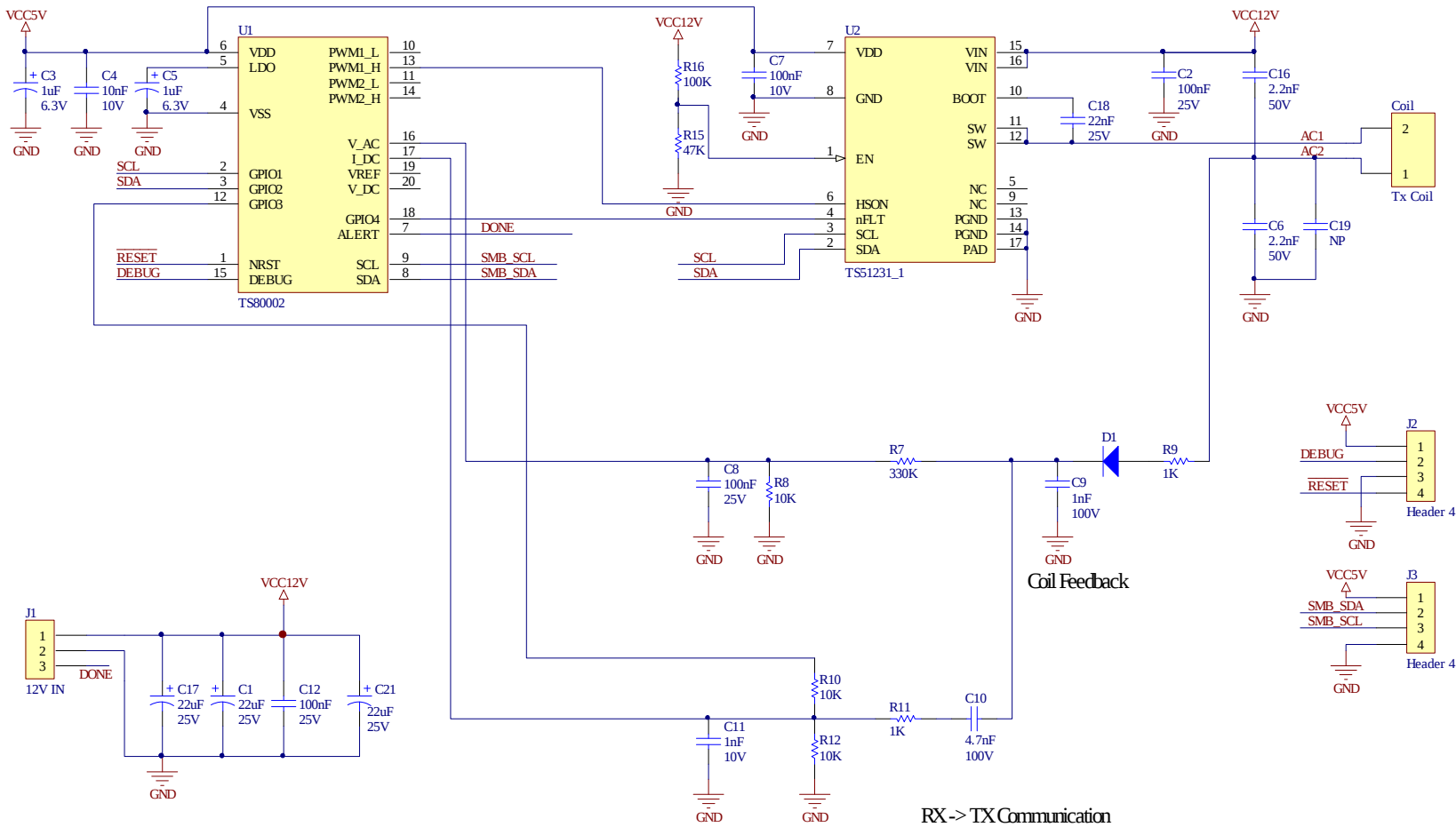
Figure 1: Schematic
