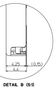
DETAIL B (5:1)
