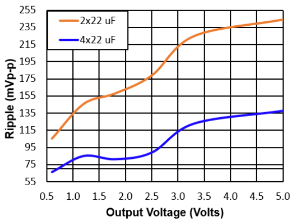
Figure 37. Input ripple voltage for various output voltages with 2x22μF or 4x22μF ceramic capacitors at the input (6A load). Input voltage is 12V.
