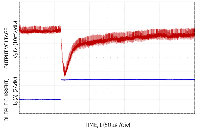
Figure 10. Transient Response to Dynamic Load Change from 50% to 100% at 12Vin, Cout-1x330µF, 4x100µF, Ctune-4.7nF, Rtune-500
