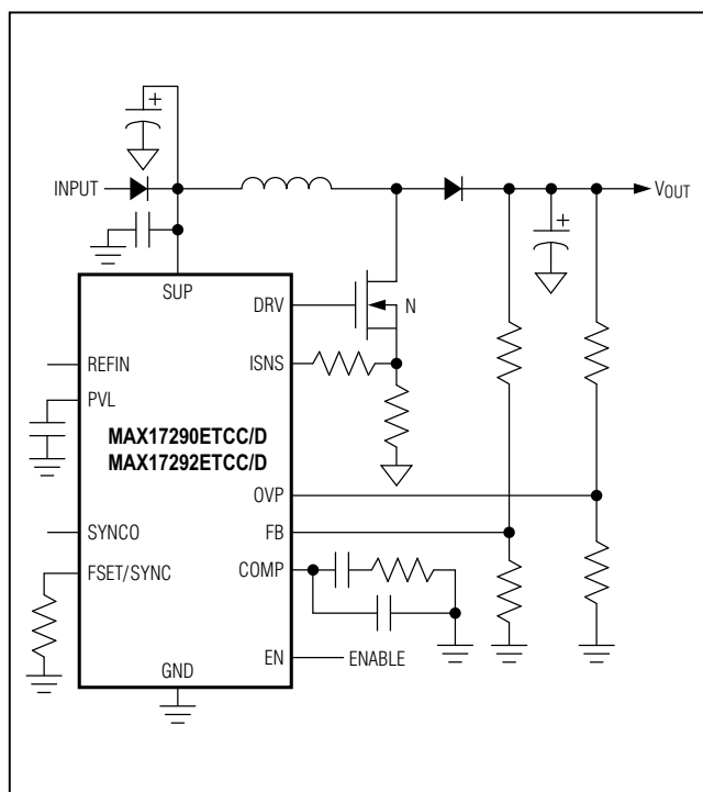
Figure 2. Application with Independent Output Overvoltage Protection
