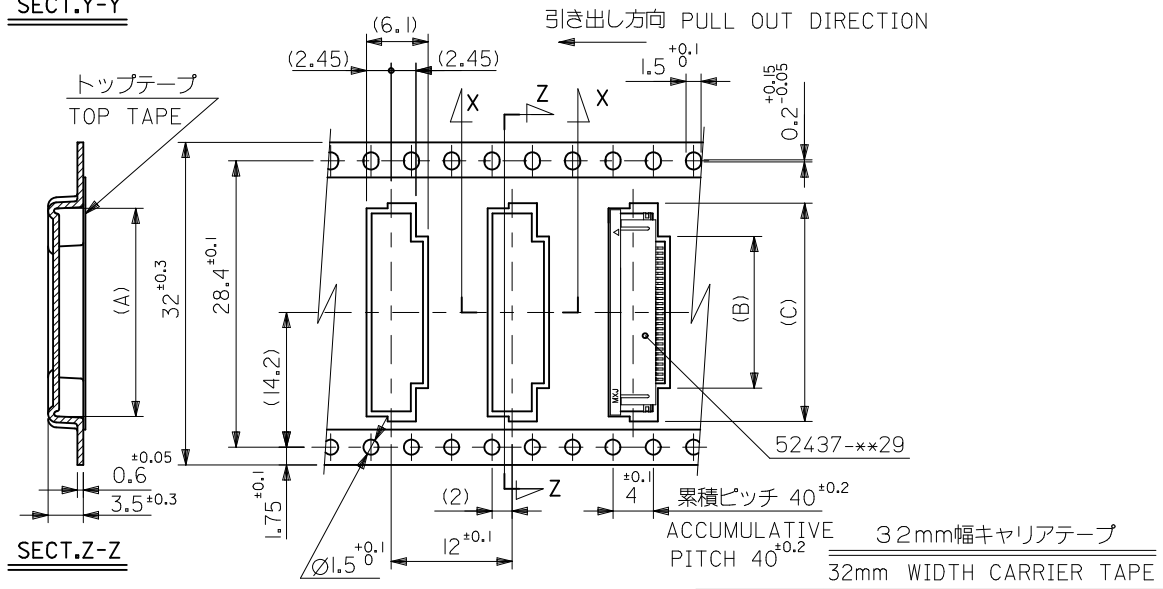
SECT.Y-Y
