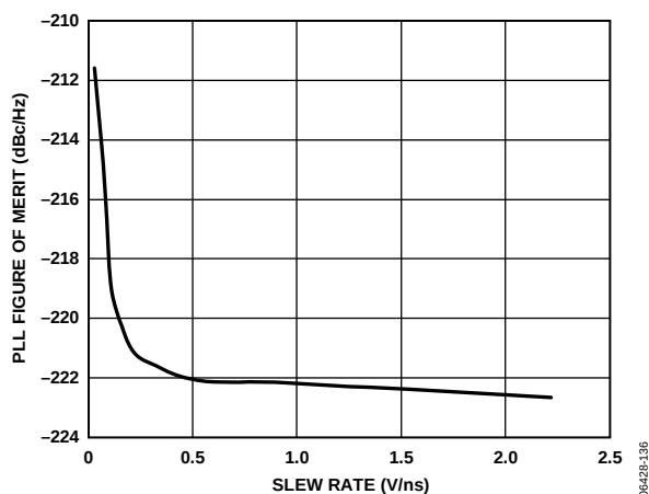
Figure 14. PLL Figure of Merit (FOM) vs. Slew Rate at \overline{\text{REFIN}}/\overline{\text{REFIN}}
