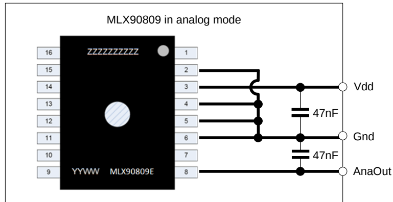
Figure 4: MLX90809 application schematic in analog mode
