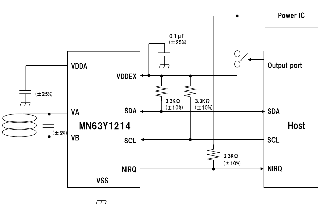
Figure 2-3 Connection Example
