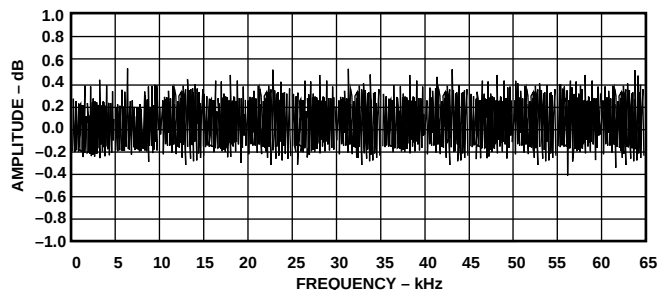
Figure 19. DNL Plot at V_{REF} = 10 \text{ V} , T_A = +25^\circ \text{C} , f_S = 100 kSPS
