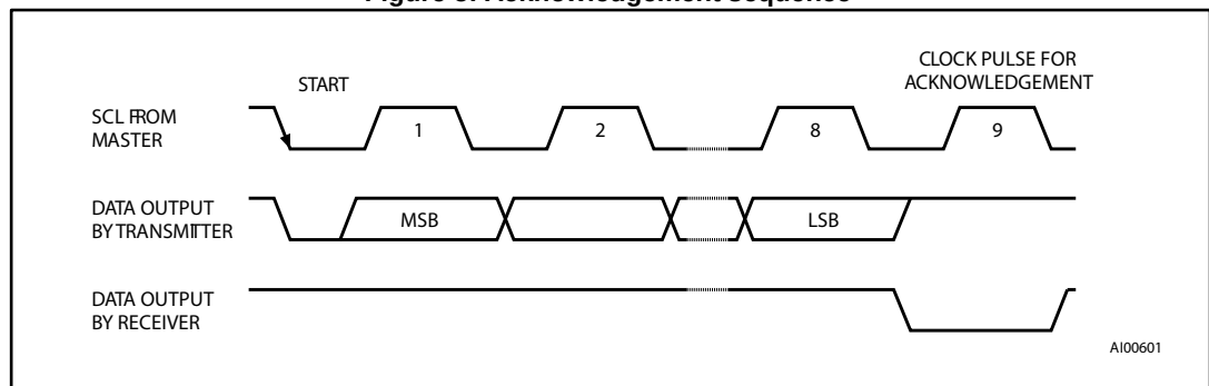
Figure 5: Acknowledgement sequence
