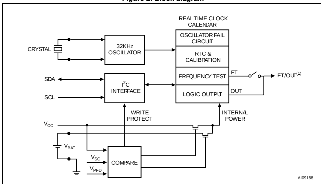
Figure 2: Block diagram
