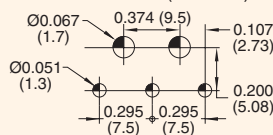
Drilling Patterns for PCB Terminals (Lateral with Location Pins) 0.024 x 0.020 (0.6 x 0.5)
