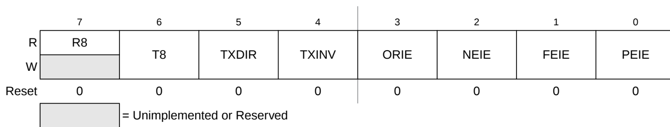
Figure 13-10. SCI Control Register 3 (SCI1C3)
