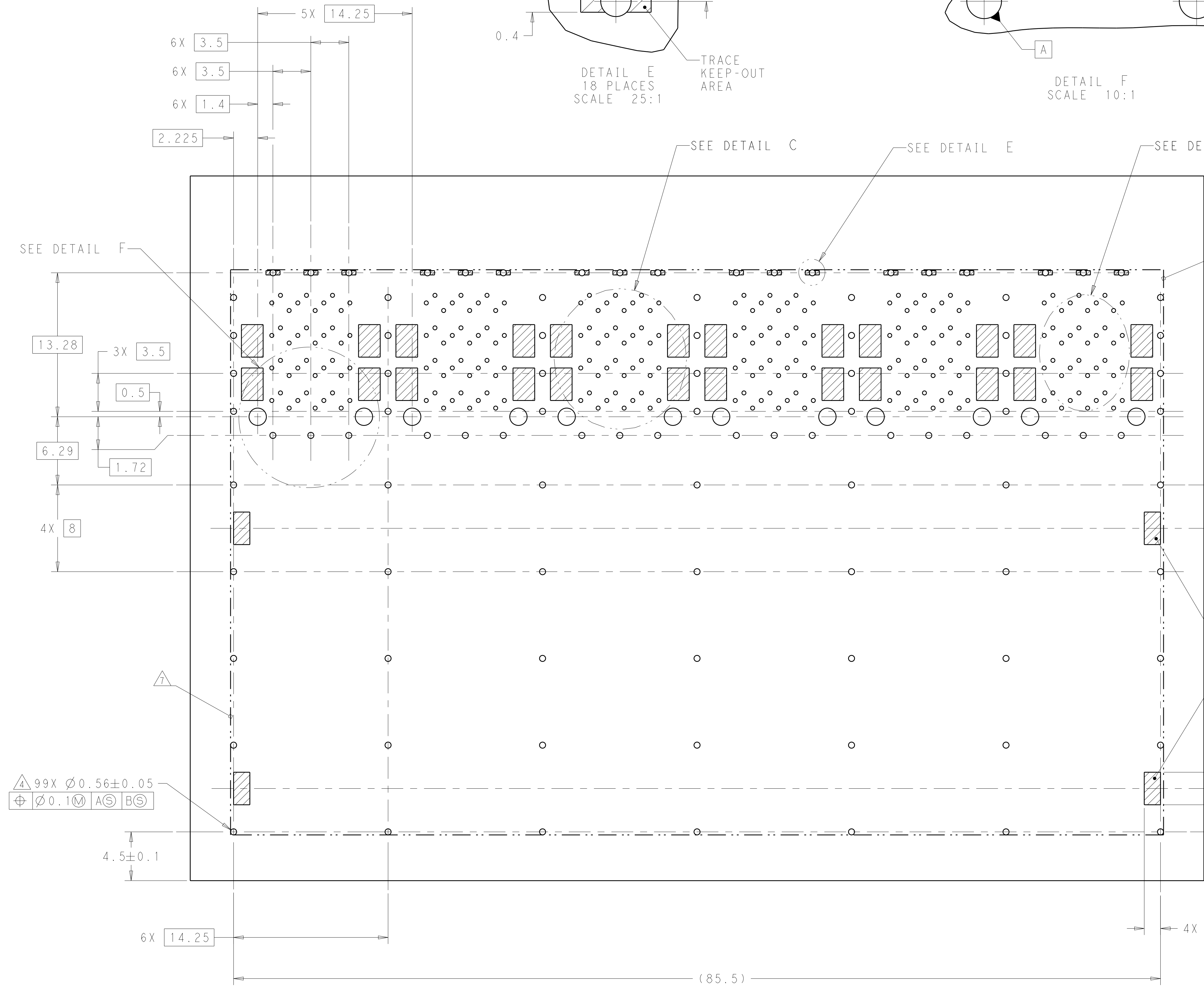
RECOMMENDED PCB LAYOUT SCALE 5:1
