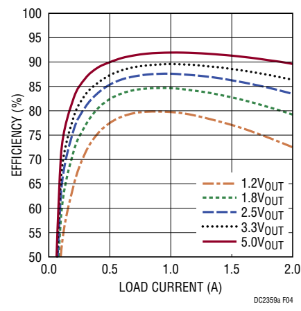
Figure 4. Forced Continuous Mode – Efficiency vs Load Current at 12VIN
