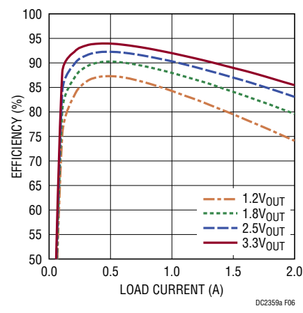
Figure 6. Forced Continuous Mode – Efficiency vs Load Current at 5VIN
