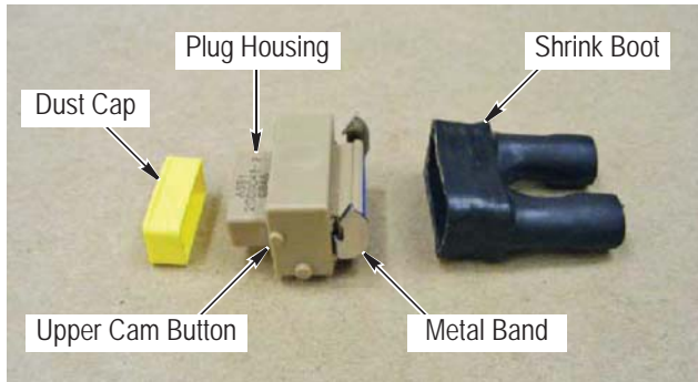
Quadrx Socket Contact Kit 2000032-1 (Quadrx Pin Contact Kits 2000031-1 and 2000031-2 Not Shown) and Quad Cable (BMS 13-72T03C04G024) 1835611-3
