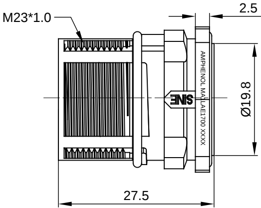
ASSEMBLED VIEW
