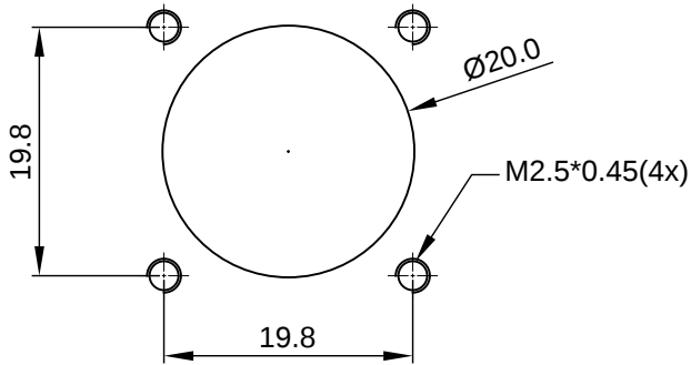
Mounting Holes
