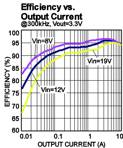
Figure 44 — Efficiency Curve
